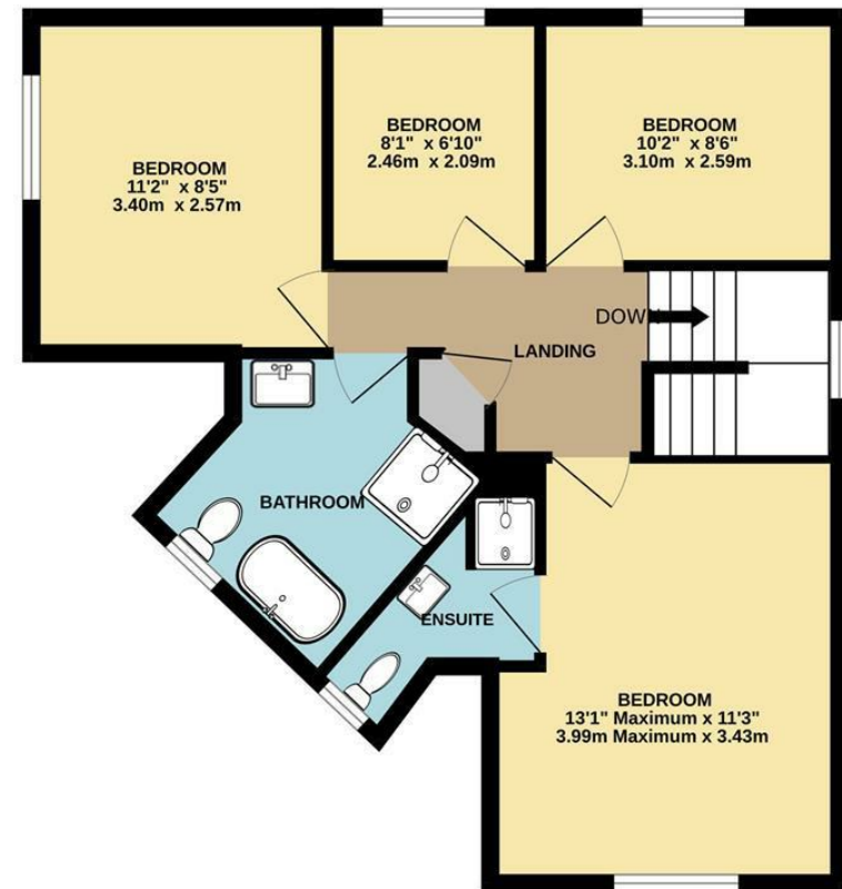
1ST FLOOR
